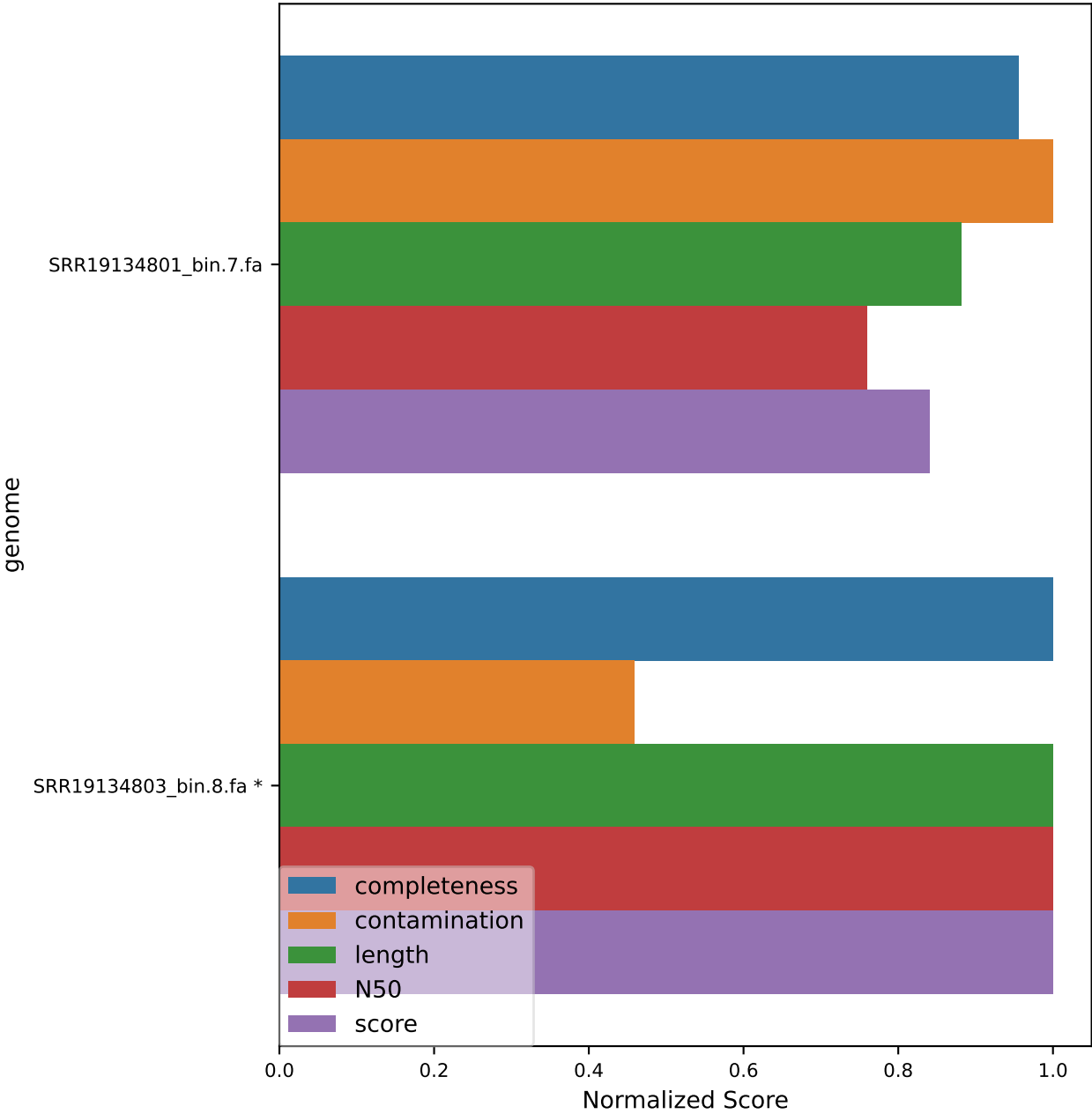
Scoring of cluster 667_1
